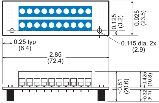
Figure C-4. FWT50 Dimensions
