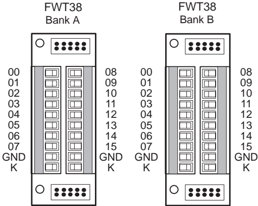
Figure C-3. FWT38 Pinouts
