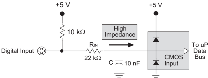
Figure B-3. Protected Input Circuitry, HVA00 through HVA15
